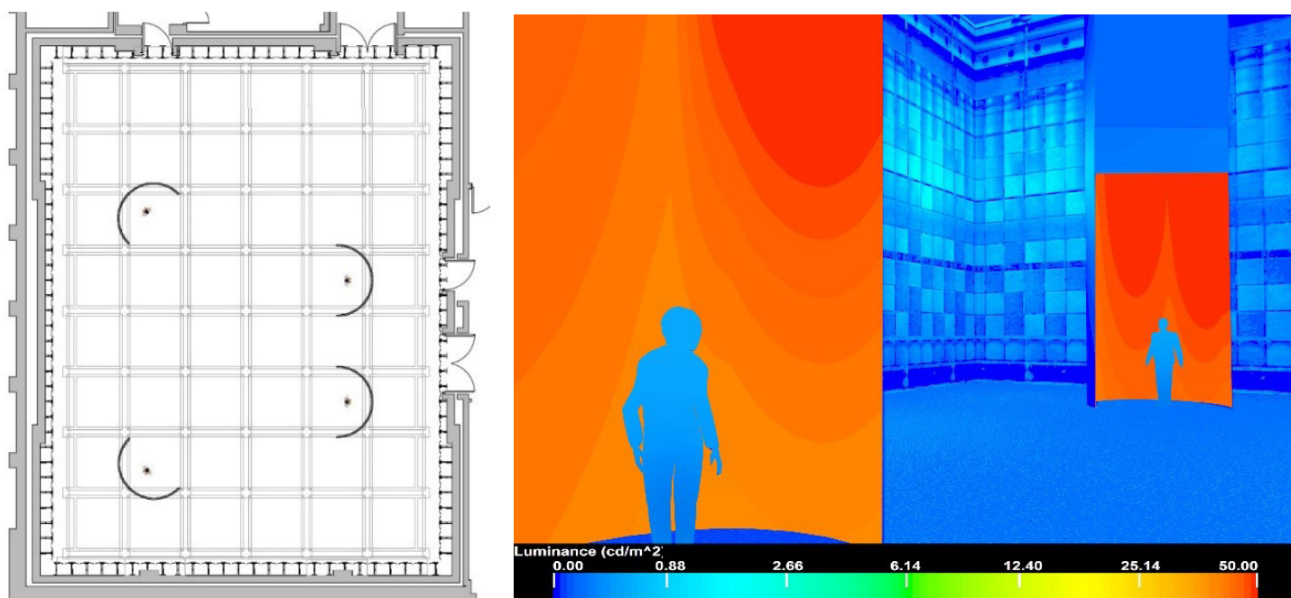
Figure 1: Layout diagram of the black-box space, with four semi-circular luminous color spaces (Left); light level and distribution simulation (Right)
