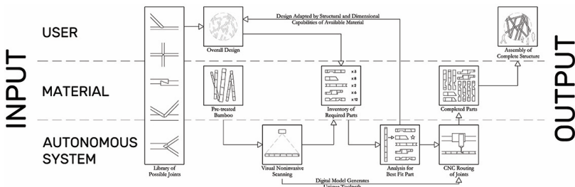
Figure 6: Integrated scanning, parametric part selection, and CNC routing machine for bamboo pole construction. Source: (Author 2019)
