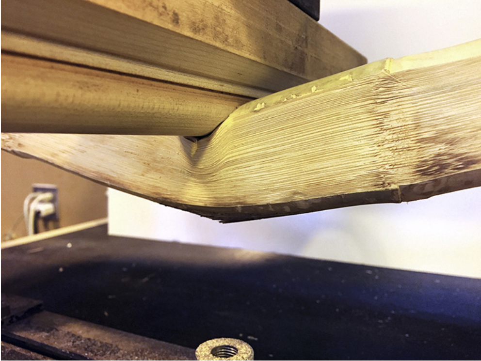
Figure 1: Uniform bending testing. Source: (Author 2019)
