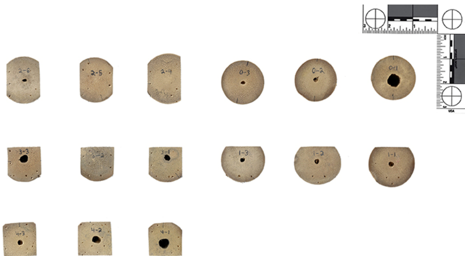
Figure 8: Cross sections of faced Calcutta Bamboo. Source: (Author 2019)
